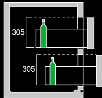
H880 2 cassetti uguali 2 identical drawers
