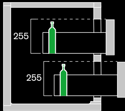
H770 2 cassetti uguali 2 identical drawers
